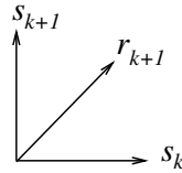
Figure 9.3: Search directions and residuals in Conjugate Gradients. The choice of \alpha_k in (9.24) insures that r_{k+1} \perp_I s_k , and the choice of \beta_k in (9.28) insures that s_{k+1} \perp_C s_k .
