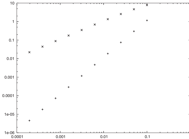
Figure 17.1: Absolute error in computing e^\pi \approx 23.141 by the explicit Euler method (16.26) (×’s) and by the centered scheme (17.1) (+’s). The horizontal axis is \Delta t , and the vertical axis is the absolute error at T = 1 .
