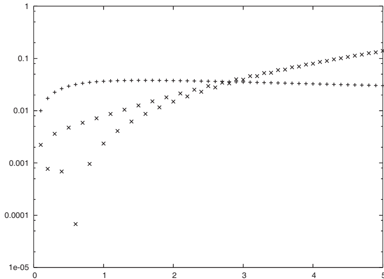
Figure 17.3: Comparison of relative absolute errors (17.2) for the centered scheme (17.1) (×'s) and the explicit Euler scheme (16.26) (+'s) for solving u' = -u^2 .
