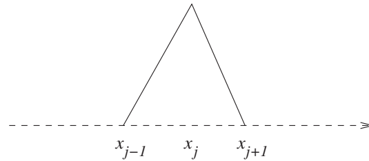
Figure 12.3: A picture of a typical basis function \phi_j for continuous, piecewise linear interpolation; \phi_j is zero outside the interval [x_{j-1}, x_{j+1}] .
