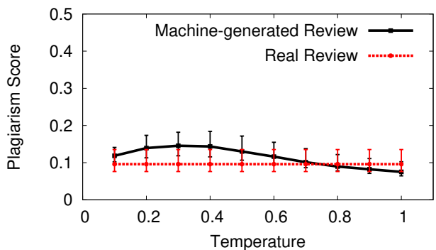
Figure 6: Plagiarism similarity score. Each point shows median, 25th and 75th percentile of the score distribution.
