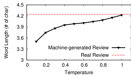
(a) Average word length (structural feature)
