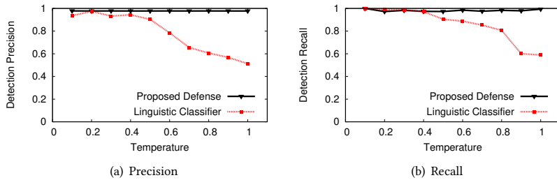
Figure 10: Performance of proposed defense and linguistic classifier (Section 4.1).
