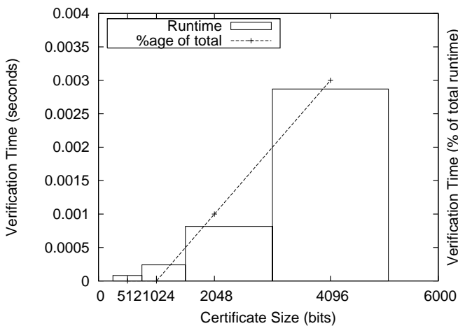
Figure 3. Certificate Runtime and Overhead
