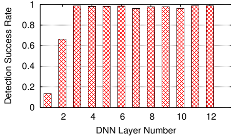
Figure 10: Detection success rate of CW attack at 5% FPR when using different layers for detection in a GTSRB model.
